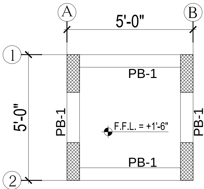
PLINTH BEAM LAYOUT PLAN
