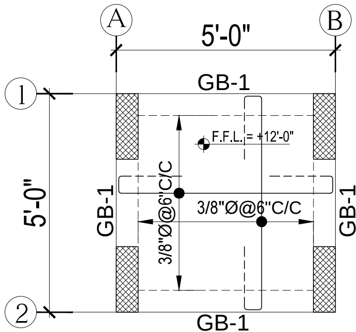
GROUND FLOOR SLAB FRAMING PLAN
