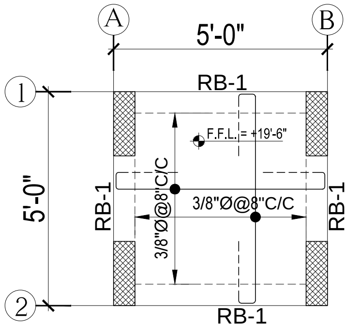
ROOF SLAB FRAMING PLAN
