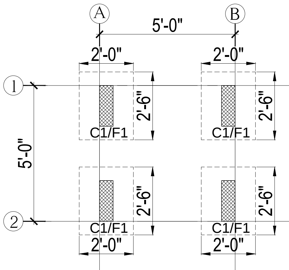
FOUNDATION LAYOUT PLAN
